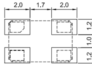
Top Perspective View Suggest Layout Units: mm
