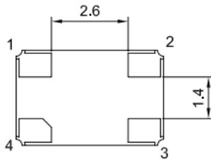
Top Perspective View
